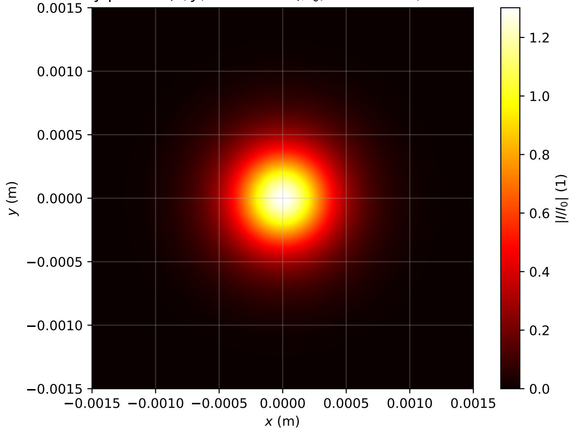
Intensity profile I(x, y, z = 1.035m)/I_0 , Pin=0.8Pcr, artificial time
